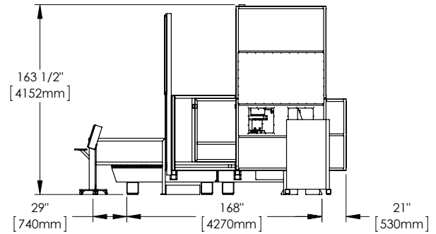
Twin 6' x 5' Shuttle Tables (pictured)
